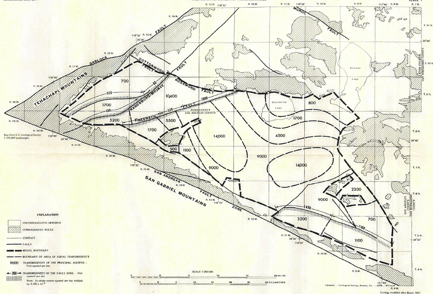
MAP OF ANTELOPE VALLEY, CALIFORNIA, SHOWING TRANSMISSIVITY USED IN THE MATHEMATICAL MODEL OF THE PRINCIPAL AQUIFER
