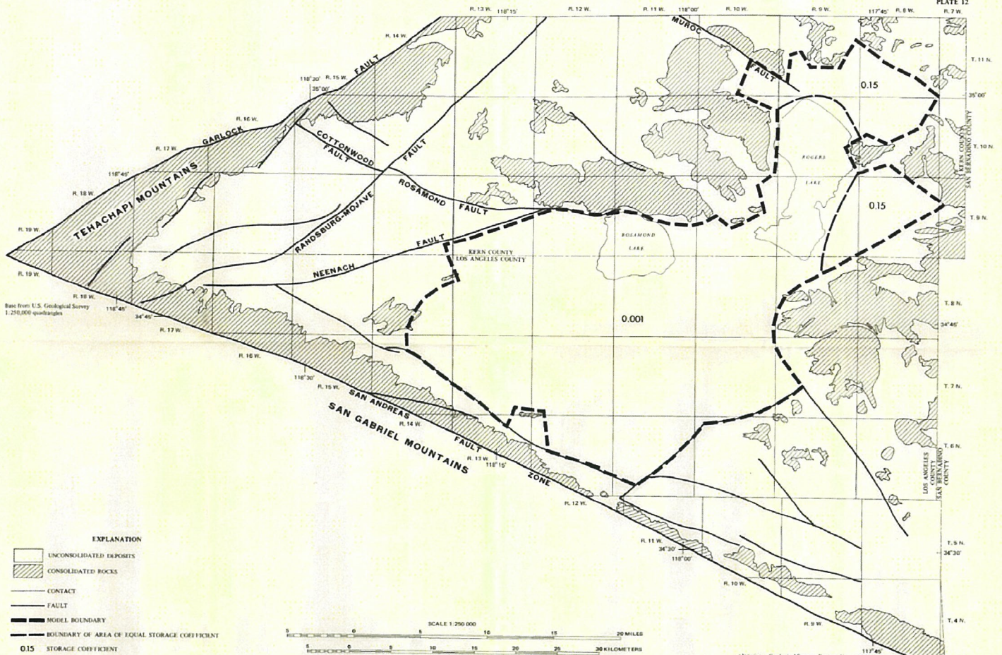
MAP OF ANTELOPE VALLEY, CALIFORNIA, SHOWING STORAGE COEFFICIENT USED IN THE MATHEMATICAL MODEL OF THE DEEP AQUIFER
