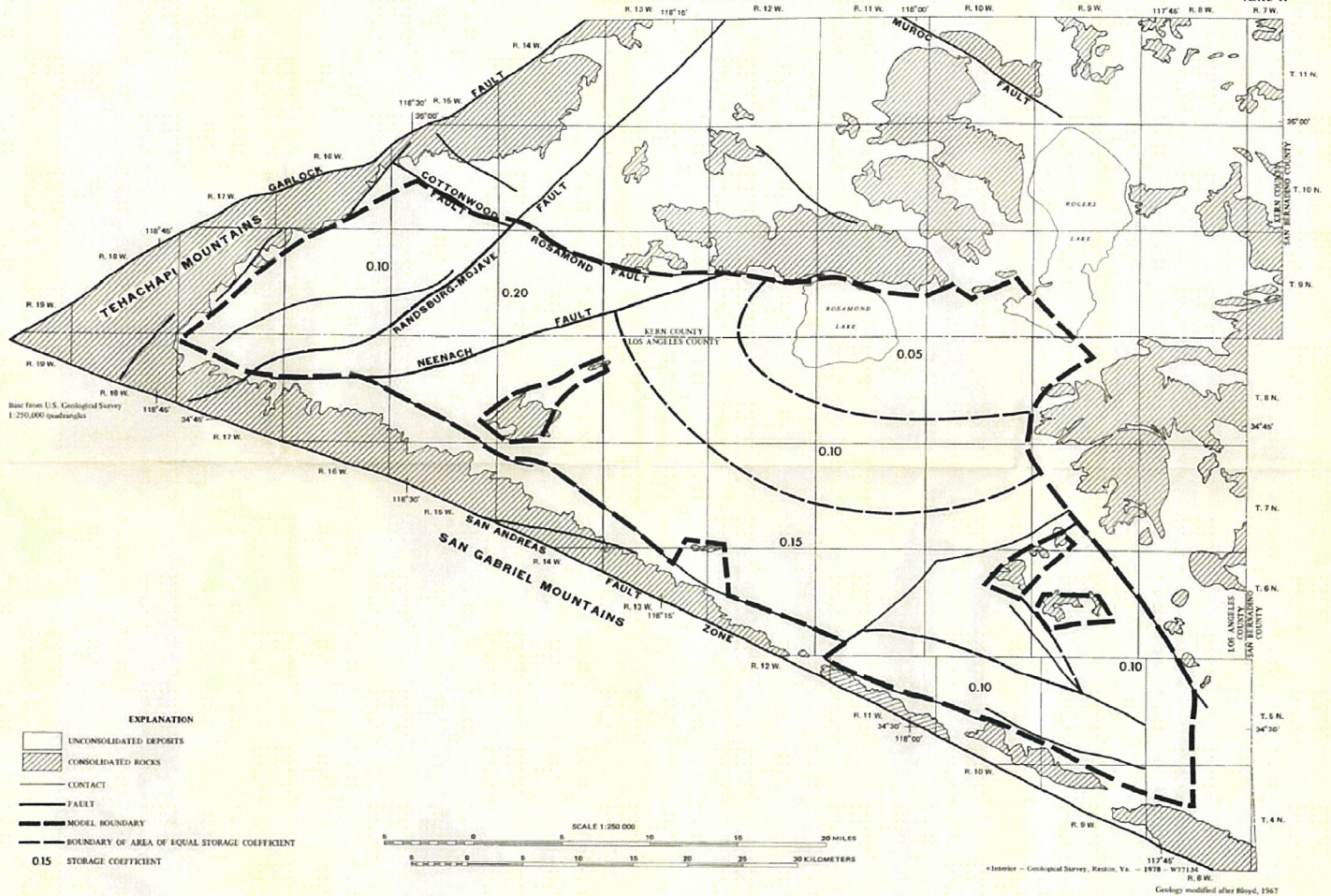
MAP OF ANTELOPE VALLEY, CALIFORNIA, SHOWING STORAGE COEFFICIENT USED IN THE MATHEMATICAL MODEL OF THE PRINCIPAL AQUIFER
