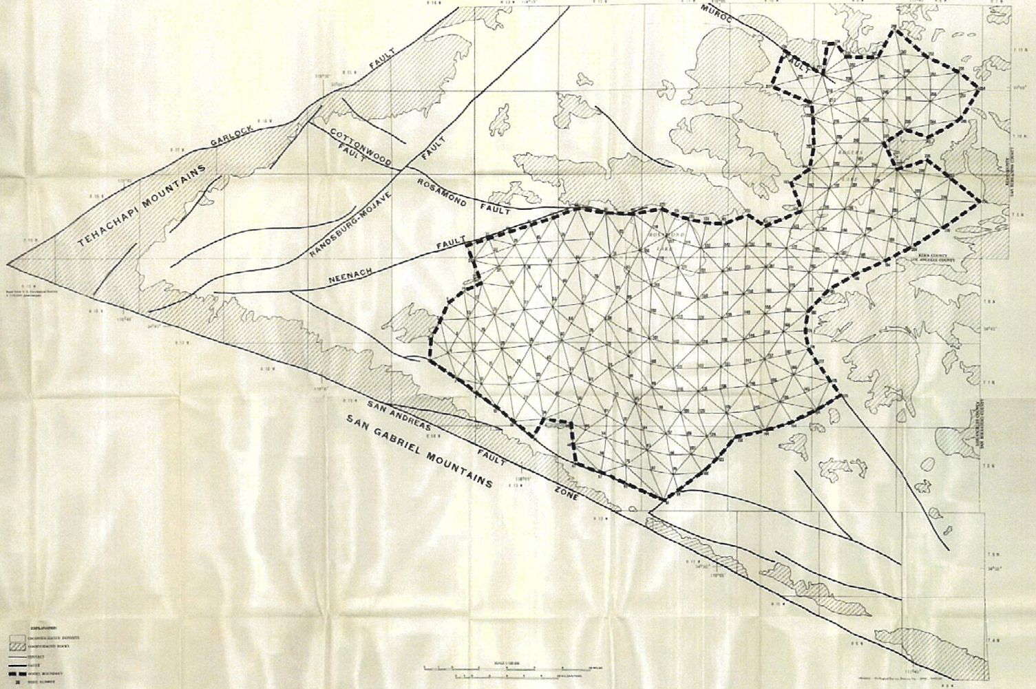
MAP OF ANTELOPE VALLEY, CALIFORNIA, SHOWING FINITE-ELEMENT CONFIGURATION USED IN THE MATHEMATICAL MODEL OF THE DEEP AQUIFER
