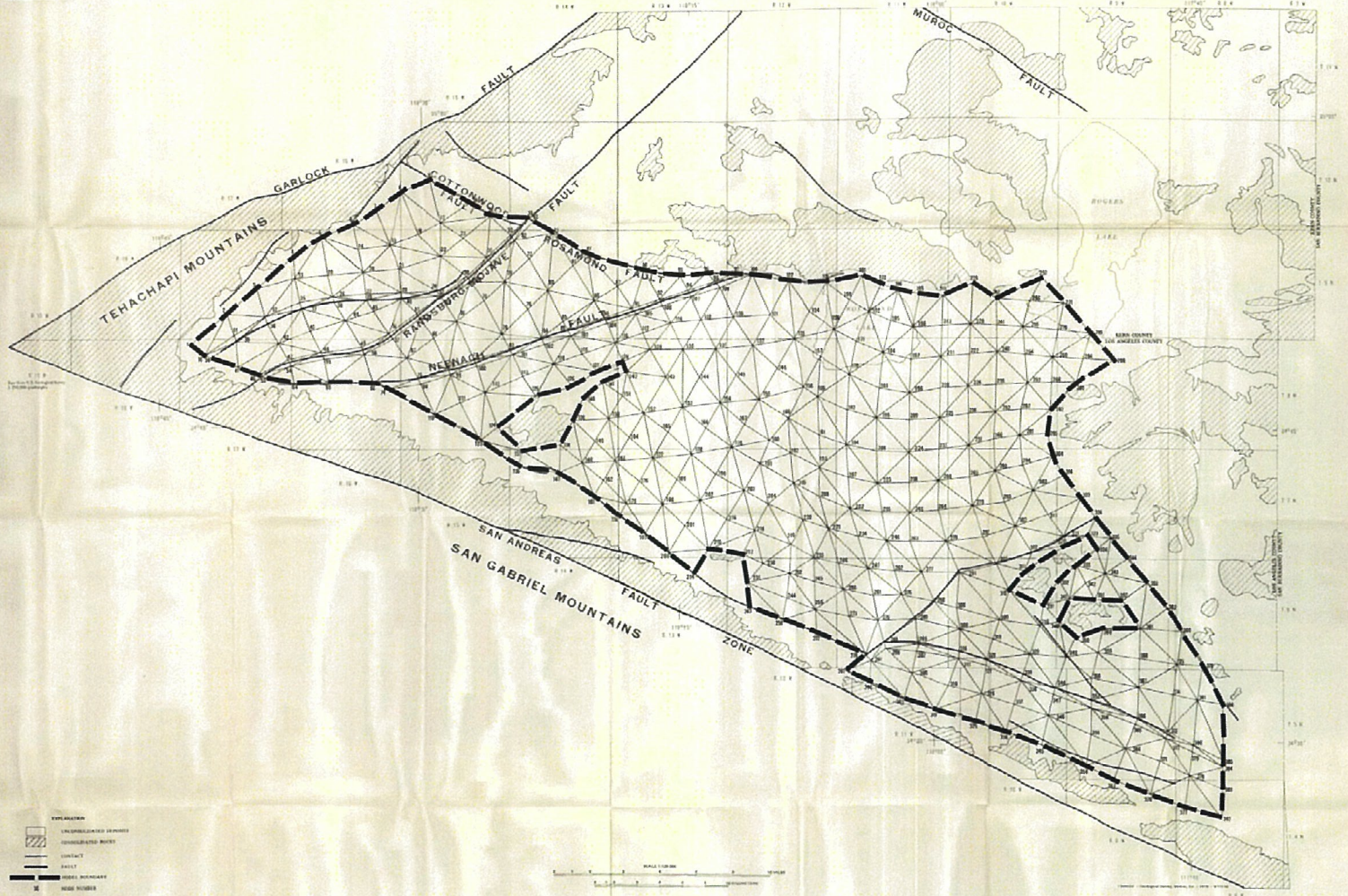
MAP OF ANTELOPE VALLEY, CALIFORNIA, SHOWING FINITE-ELEMENT CONFIGURATION USED IN THE MATHEMATICAL MODEL OF THE PRINCIPAL AQUIFER
