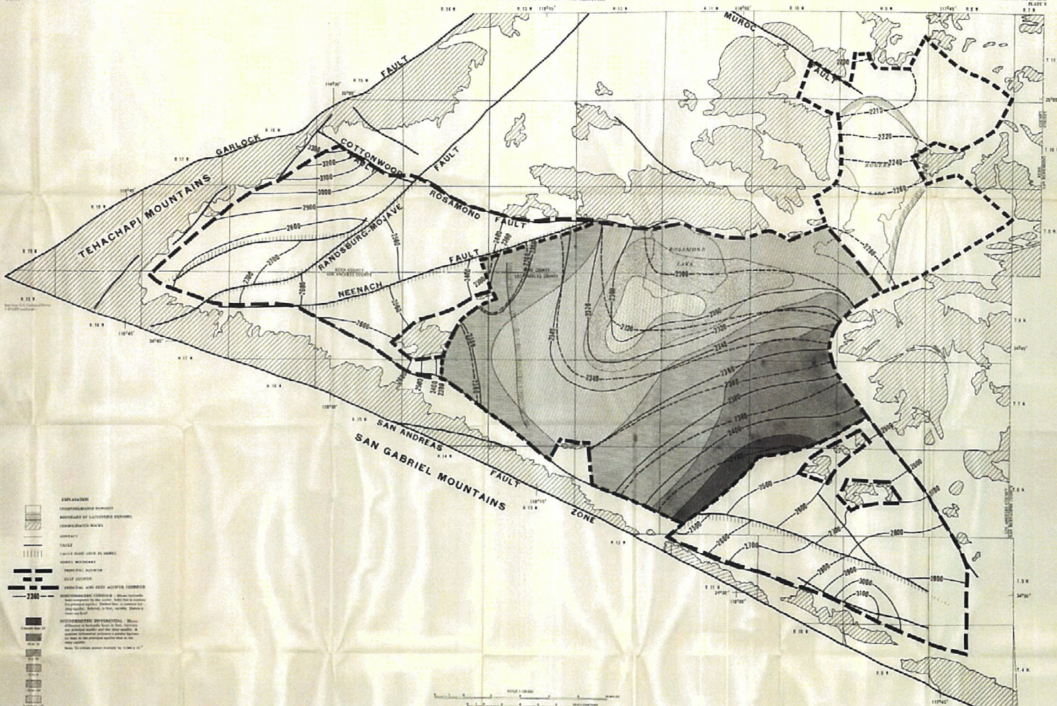
POTENTIOMETRIC MAP FOR 1955 COMPUTED BY THE MATHEMATICAL MODEL OF THE PRINCIPAL AND DEEP AQUIFERS, ANTELOPE VALLEY, CALIFORNIA
