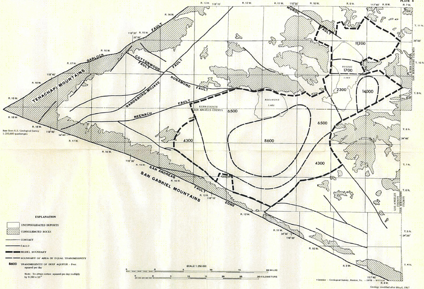
MAP OF ANTELOPE VALLEY, CALIFORNIA, SHOWING TRANSMISSIVITY USED IN THE MATHEMATICAL MODEL OF THE DEEP AQUIFER
