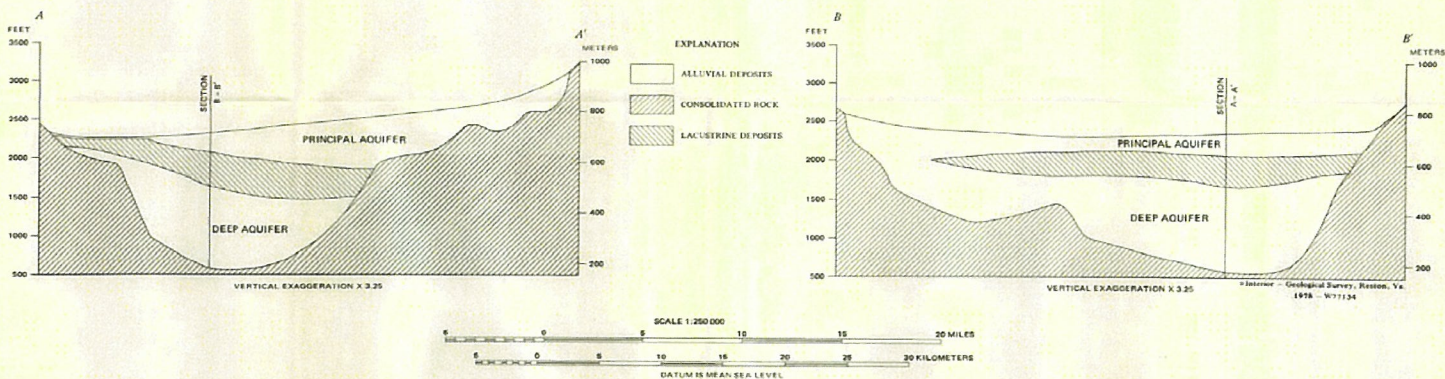
MAP OF ANTELOPE VALLEY, CALIFORNIA, SHOWING GEOGRAPHIC SETTING, GENERALIZED GEOLOGY, BOUNDARIES USED IN THE MATHEMATICAL MODEL, AND GEOLOGIC SECTIONS THROUGH THE GROUND-WATER BASIN
