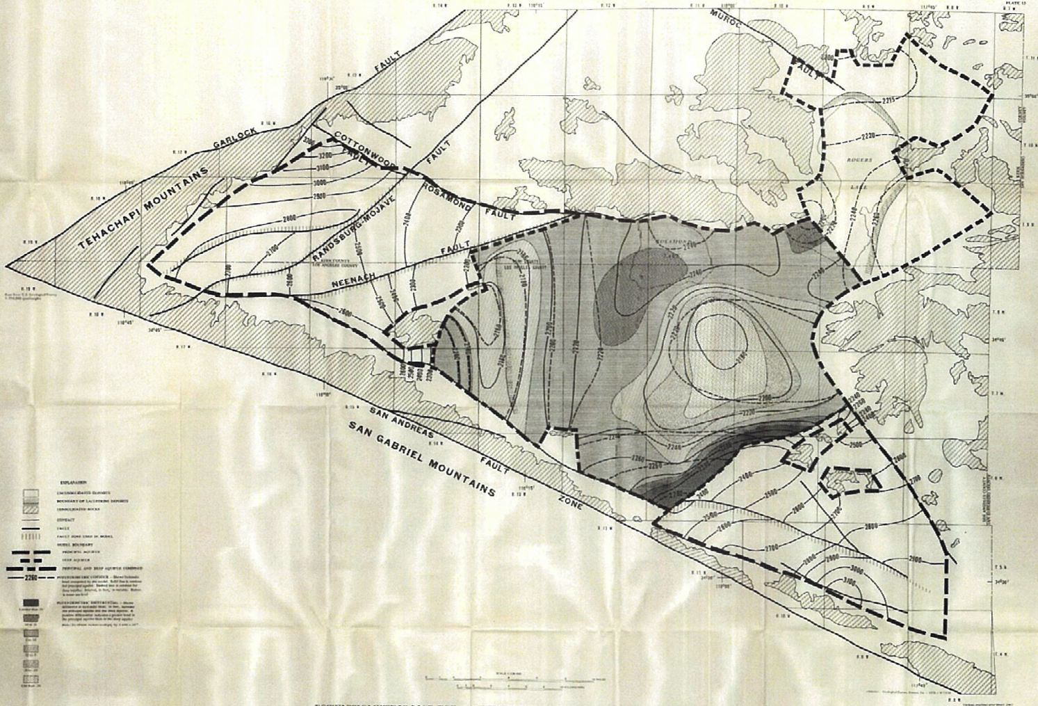
POTENTIOMETRIC MAP FOR 1961 COMPUTED BY THE MATHEMATICAL MODEL OF THE PRINCIPAL AND DEEP AQUIFERS, ANTELOPE VALLEY, CALIFORNIA
