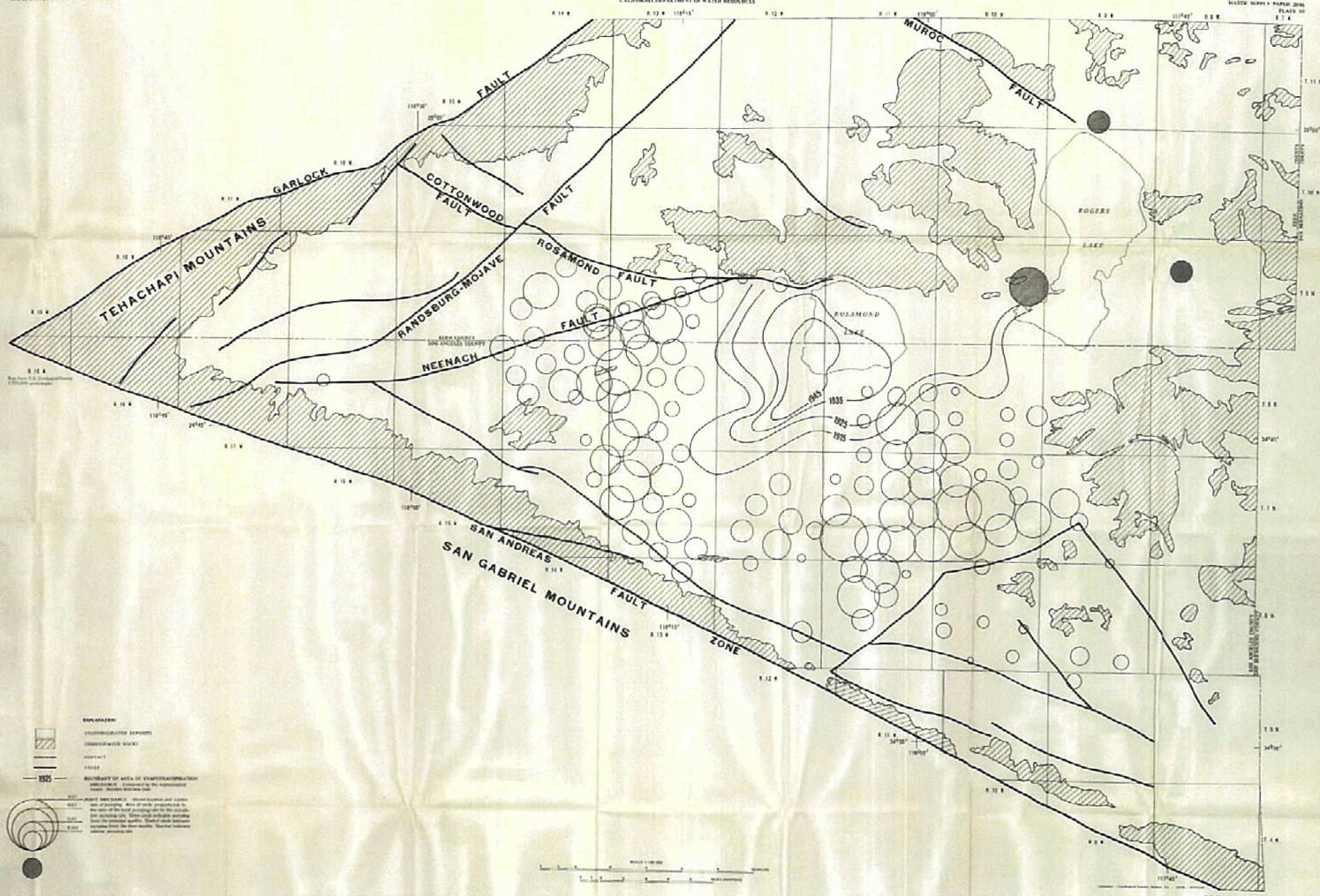
MAP OF ANTELOPE VALLEY, CALIFORNIA, SHOWING RELATIVE GEOGRAPHIC DISTRIBUTION OF PUMPAGE FROM THE PRINCIPAL AND DEEP AQUIFERS USED IN THE MATHEMATICAL MODEL FOR 1915 THROUGH 1961
